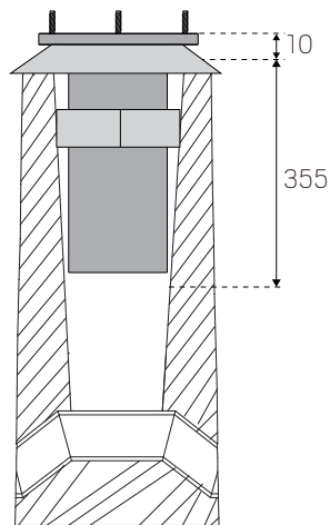
Foundation 365 Installation depth 355mm
