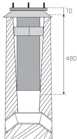
Foundation 490 Installation depth 480mm
