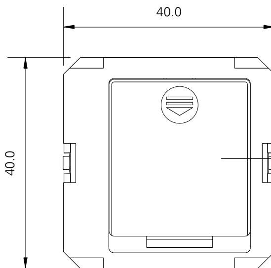
Back side
